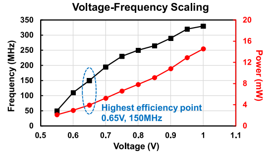
Fig. 17. ETCIM's voltage–frequency scaling curves.
