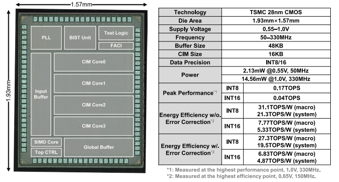
Fig. 16. ETCIM's chip micrograph and specifications.
