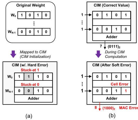
Fig. 1. (a) Hard and (b) soft error mechanisms in digital CIM.
