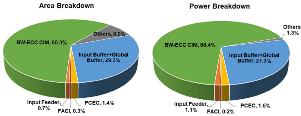
Fig. 19. ETCIM's area and power breakdown.
