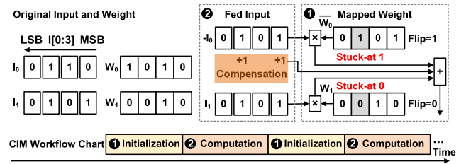
Fig. 6. Hard error repair workflow example. ① Weights are adaptively flipped to match faulty SRAM cells’ distribution in CIM initialization. ② Inputs are inverted accordingly in CIM computation.
