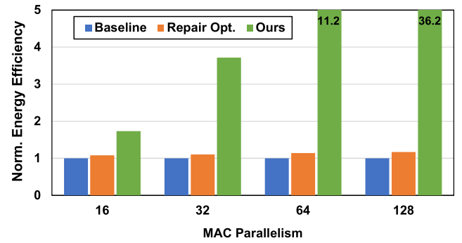
Fig. 23. Energy efficiency improvement breakdown of different techniques under various MAC parallelisms. SER is 1E-5 . "Baseline": digital CIM with only redundant column repair and BW-ECC for hard and soft error corrections. "Repair Opt.": baseline + redundancy-free repair. "Ours": baseline + redundancy-free repair + run-time cell error correction.
