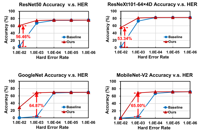
Fig. 21. Accuracy improvement from redundancy-free hard error repair on various benchmarks.
