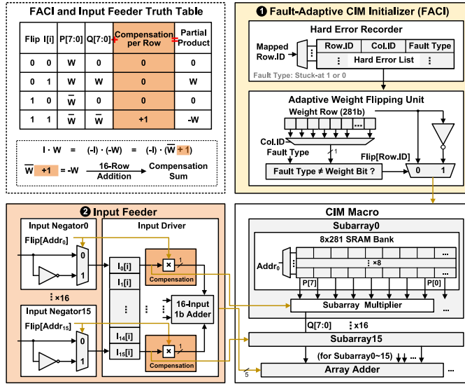
Fig. 7. FACI and input feeder architecture.
