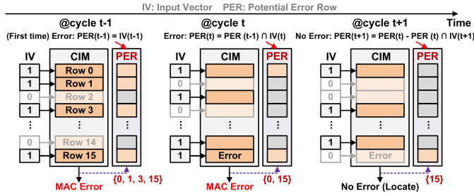
Fig. 12. Soft cell error correction example (error row = row 15).
