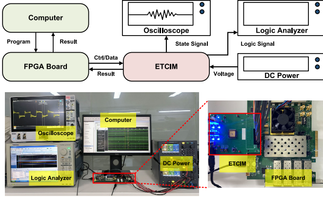
Fig. 20. Test platforms for the fabricated ETCIM processor.
