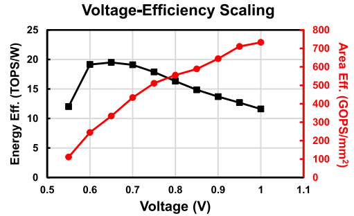
Fig. 18. ETCIM's voltage–efficiency scaling curves. The energy and area efficiency are plotted at INT8 precision.
