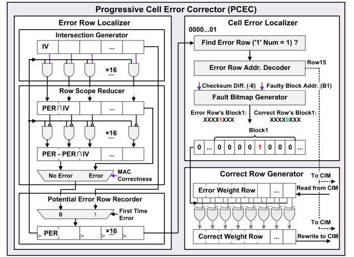
Fig. 14. PCEC architecture.
