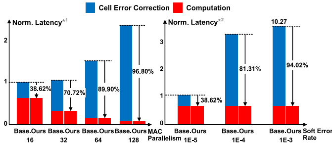
Fig. 15. Evaluation for the PCEC on hiding soft cell error correction latency, evaluated on ResNet-50 inference at INT8. Baseline: digital CIM with BW-ECC but without PCEC, which stalls computation and reads out SRAM rows in turn to locate the error row after detecting an MAC error. *1: SER is 1E-5. *2: the MAC parallelism is 16.
