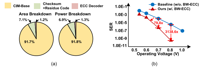
Fig. 11. Evaluation for the BW-ECC CIM on soft MAC error correction. (a) ECC code and ECC decoder overhead in a BW-ECC CIM macro. (b) SER reduction at different voltages. Baseline: conventional digital CIM without BW-ECC.
