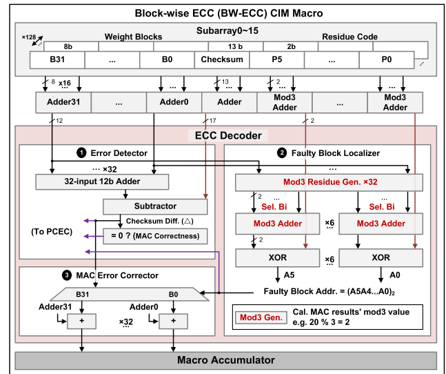
Fig. 10. BW-ECC CIM macro architecture: ❶ error detector, ❷ faulty block localizer, and ❸ MAC error corrector.
