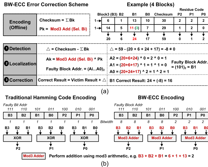
Fig. 9. Soft MAC error correction workflow. (a) BW-ECC error correction scheme and a four-block example. ❶ Error detection, ❷ faulty block localization, and ❸ error correction. (b) Comparison between traditional hamming code and our BW-ECC.
