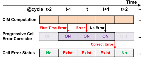
Fig. 13. Soft error correction workflow chart.
