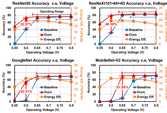
Fig. 22. Accuracy improvement from run-time soft MAC and cell error correction on various benchmarks, and operating range comparison between baseline and ours. Operating range: the effective working voltage region of digital CIM, where the inference accuracy loss is lower than 1%.
