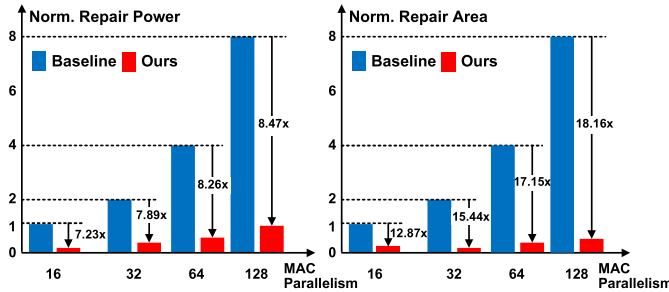
Fig. 8. Evaluation for the FACI and input feeder on hard error repair overhead reduction. Baseline: conventional column repair method, where each read-out row in digital CIM has a redundant column and detour logic for repair. MAC parallelism is the count of weight rows that are simultaneously read out and accumulated to complete MAC operations.
