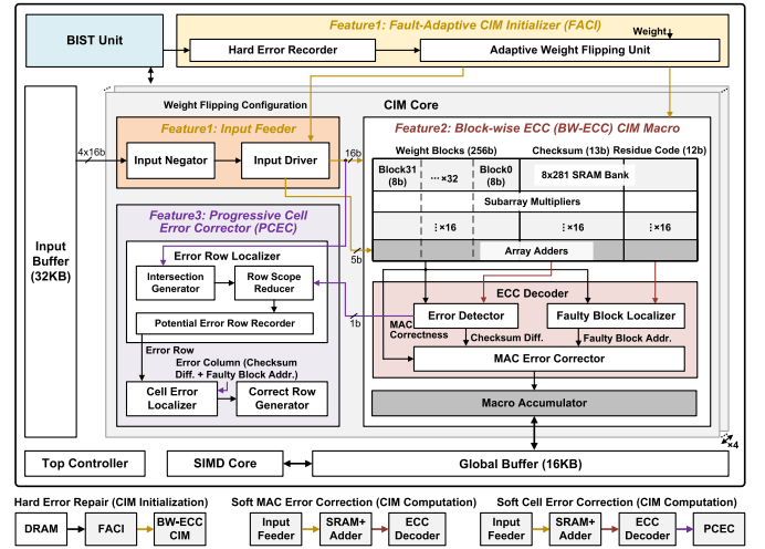
Fig. 5. ETCIM processor's overall architecture, with three configurations for hard error repair, soft MAC error correction, and soft cell error correction.
